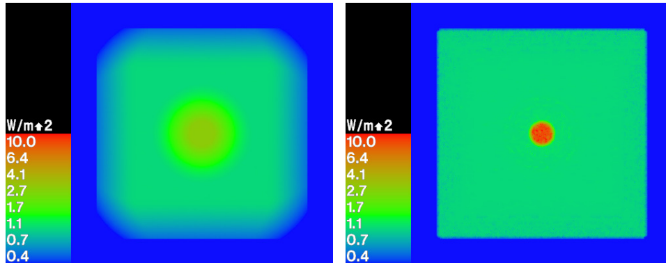
Figure 5: Left: falsecolour rendering of severely biased caustic with a bandwidth of 5000 photons. The caustic should have an irradiance of 10 \text{ W}/\text{m}^2 . Right: falsecolour rendering of the same caustic with bias compensation using a bandwidth of 50–5000 photons.
